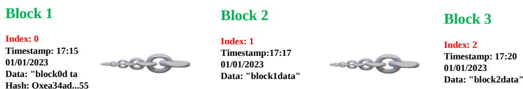
Figure 1. Blockchain structure
